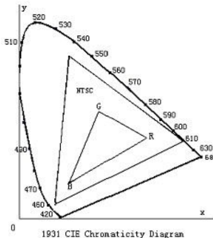
1931 CIE Chromaticity Diagram
